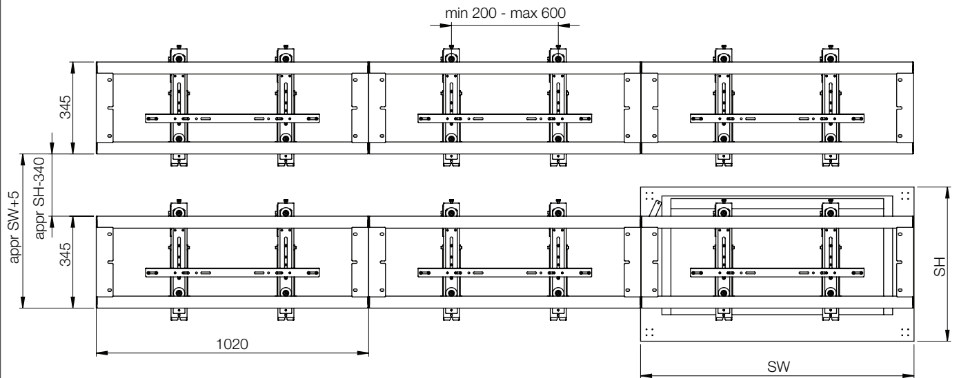
Fig. 2.1 - SMS Multi Display Wall Ace Video Row - 46/47 inch - Landscape
