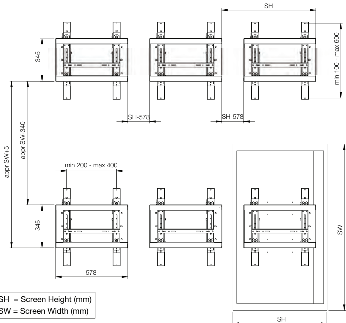
Fig. 3.3 - SMS Multi Display Wall Ace Video Row - 60 inch - Portrait
