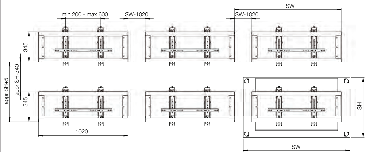
Fig 2.2 - SMS Multi Display Wall Ace Video Row - 55 inch - Landscape
