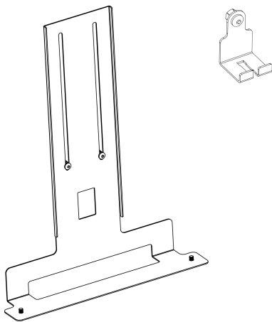
Crestron Side Shelf
