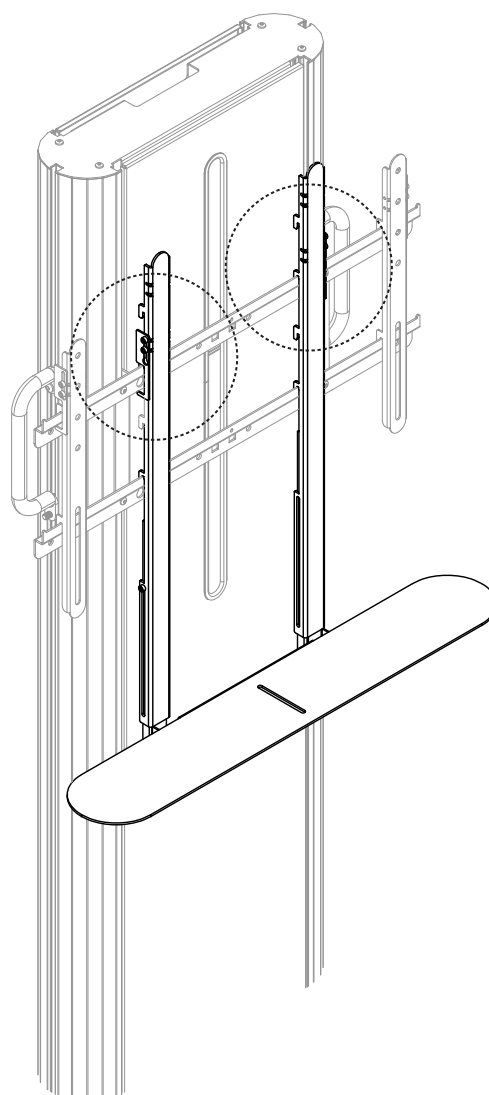
Bracket position Alt. 2
