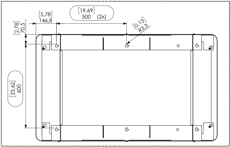
15-002-x Casing Specific Landscape 55 for Samsung OH dimensions
