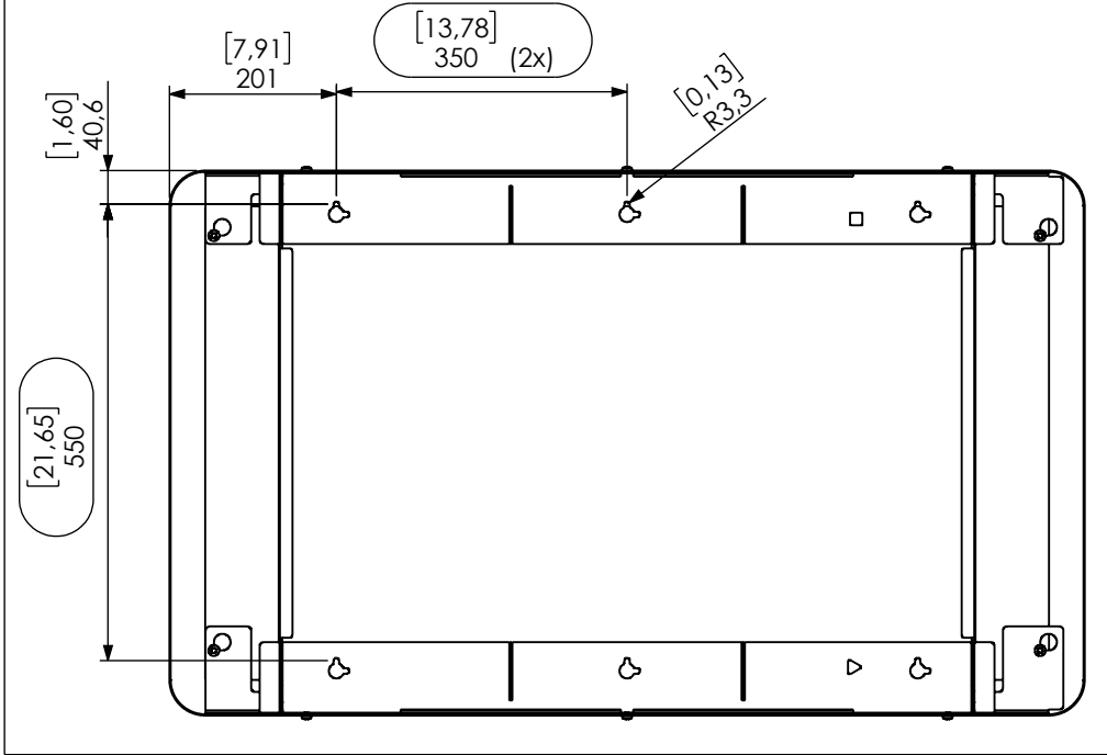
TS22024-01..15-001-x Casing Specific Landscape 46 for Samsung OH dimensions
