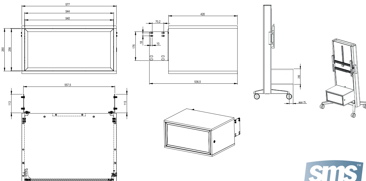
Technical drawing (mm) PR400001..PR400003 SMS Presence Media Box
