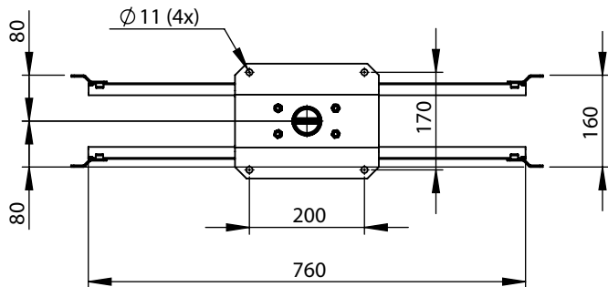
Swivel +/- 180 degrees
