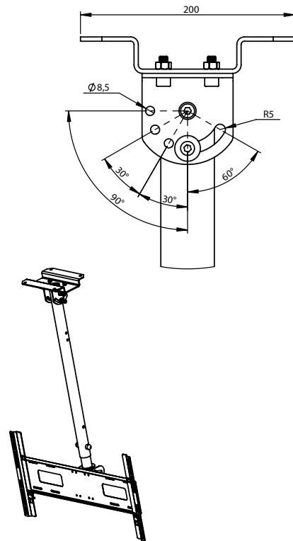
DETAIL A SCALE 1 : 3
